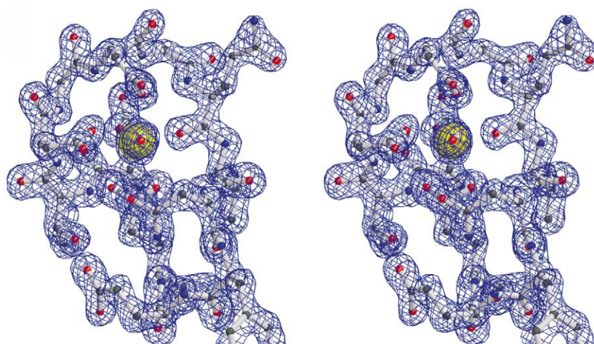
Fig. 1. Stereoview of the 2|F_o|-|F_c| electron density map in one of the \text{Ca}^{2+} binding regions (residues 129–140) contoured at 1.5\sigma . \text{Ca}^{2+} ion is represented as a yellow ball.
